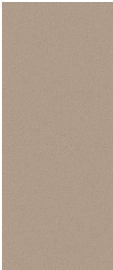
PP 2502 Dune
